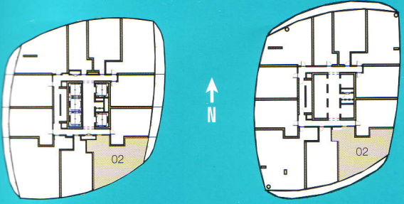
Floors 3-29
